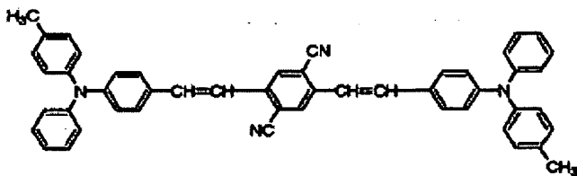
Structural formula (15)-2:
